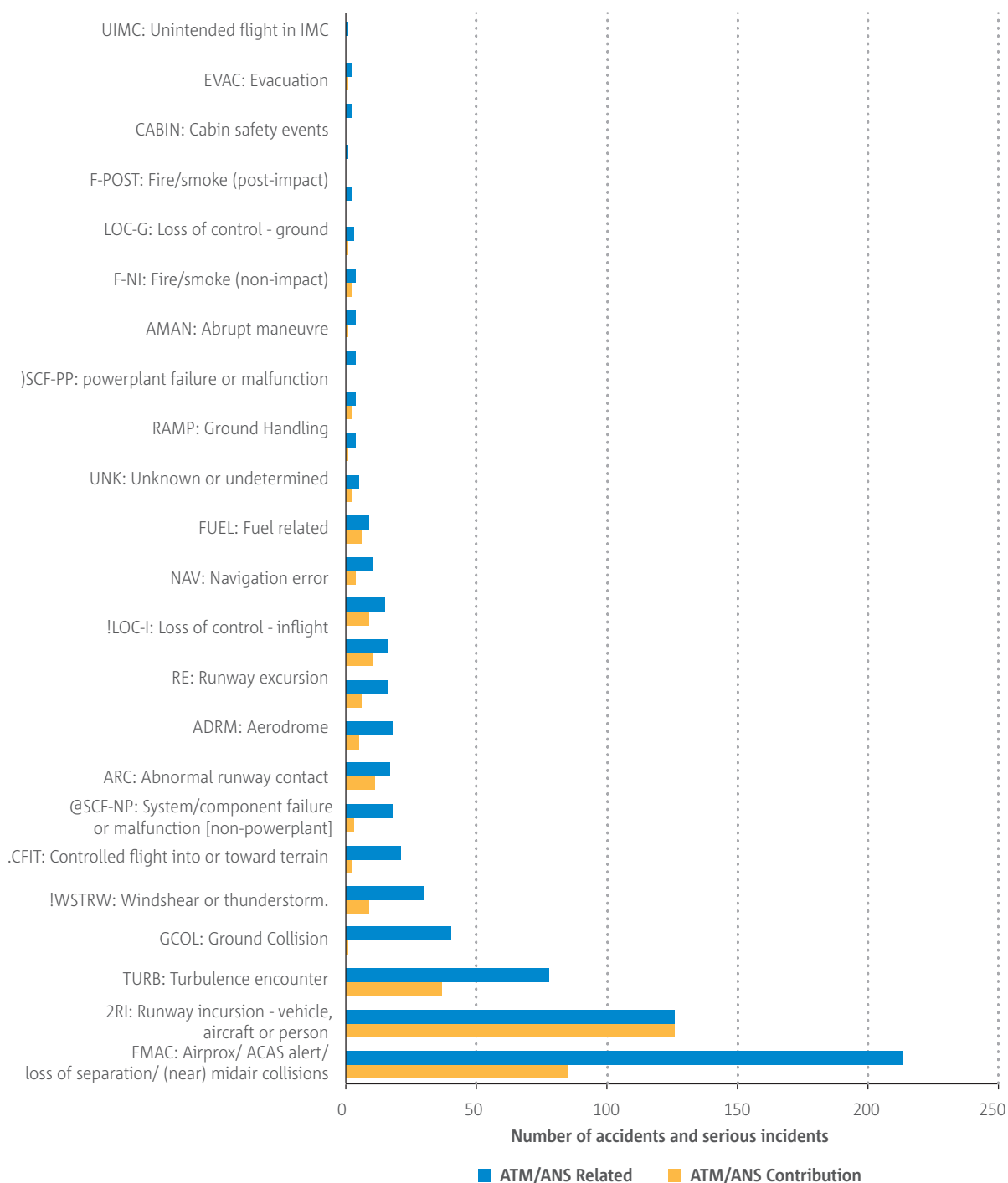
► Figure 38 ATM/ANS-related accidents and serious incidents, and those with ATM/ANS contribution during 2006-2016
