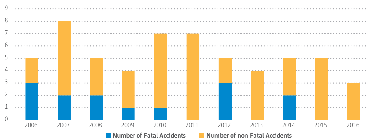
► Figure 9 Other CAT Aeroplane, evolution of fatal and non-fatal accidents (2006-2016)
