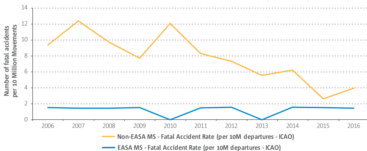
► Figure 2 CAT Aeroplane Airline fatal accident rate for EASA MS AOC and non-EASA Ms, period 2006-2016
