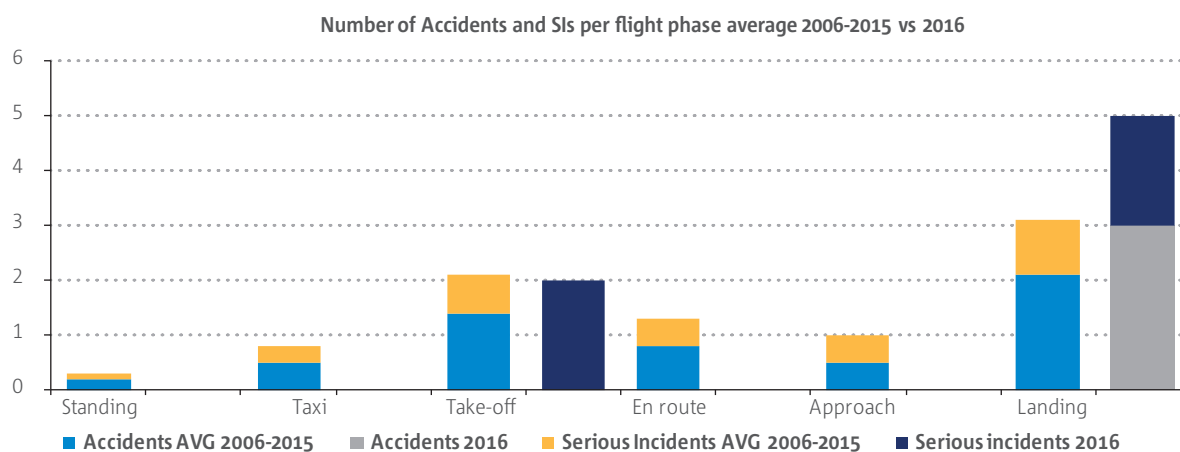
► Figure 10 Other CAT Aeroplane, comparison of accidents and serious incidents by flight phase between the average of 2006-2015 and the figures in 2016
