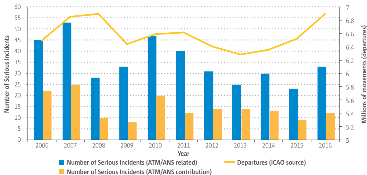
► Figure 35 ATM/ANS related serious incidents and ATM/ANS contribution per year, 2006-2016, in EASA MS
