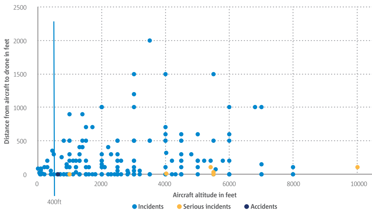
► Figure 31 Aircraft altitude vs. distance from drone at the time of detection 2010-2016
